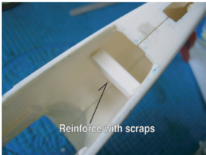
胴体の補強 Fuselage reinforcement
