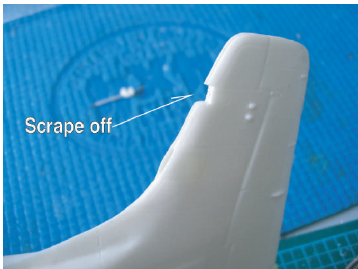
ACL 付きピトー管の取り付け -1 Installation of a pitot tube with ACL -1
